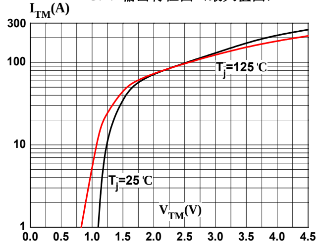
FIG.4: Output characteristic graph (maximum value graph). A graph showing I_{TM}(A) on the y-axis (1 to 300) and V_{TM}(V) on the x-axis (0.0 to 4.5) on a logarithmic scale. Two curves are shown for T_j=25^{\circ}C (black) and T_j=125^{\circ}C (red).
