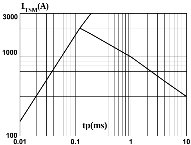
FIG.5: Non-repeating peak surge current vs. sine wave pulse width relationship curve. A graph showing I_{TSM}(A) on the y-axis (100 to 3000) and tp(ms) on the x-axis (0.01 to 10) on a logarithmic scale. The current increases with pulse width up to 0.1ms and then decreases.
