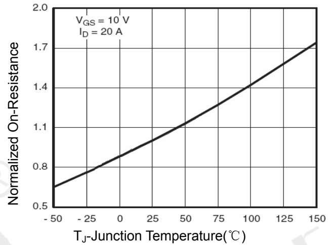
Figure 4 Rdson-Junction Temperature
